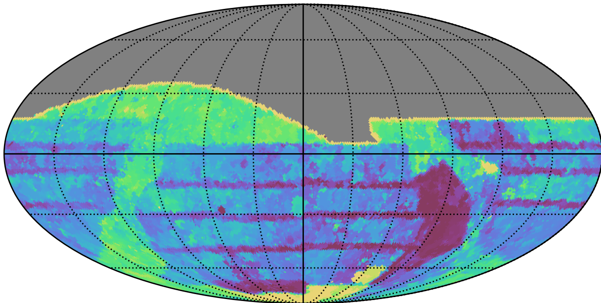
baseline_v2.0_10yrs All sky all bands: Max Inter-Night Gap
