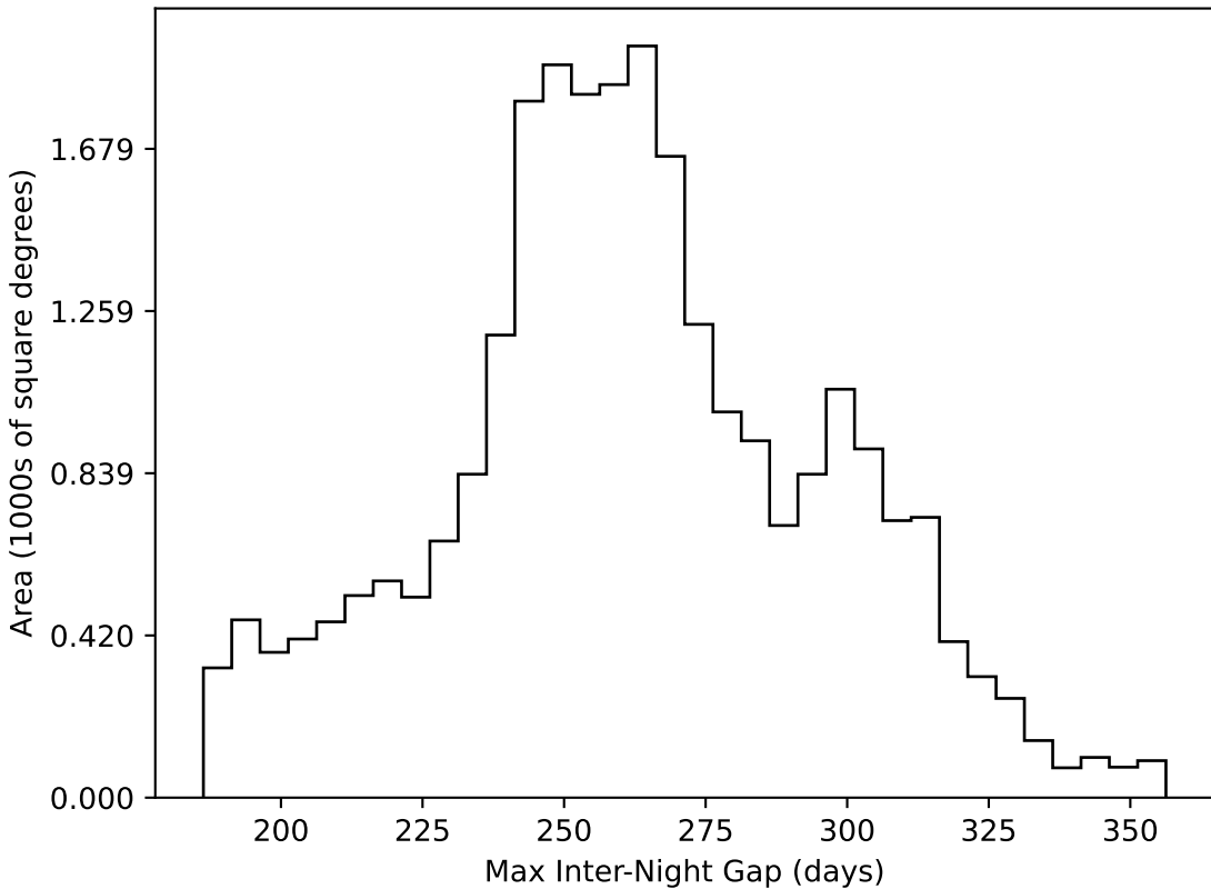
baseline_v2.0_10yrs All sky all bands: Max Inter-Night Gap
