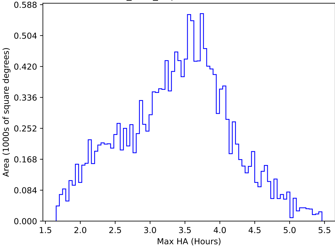
baseline_v2.0_10yrs WFD u band: Max HA
