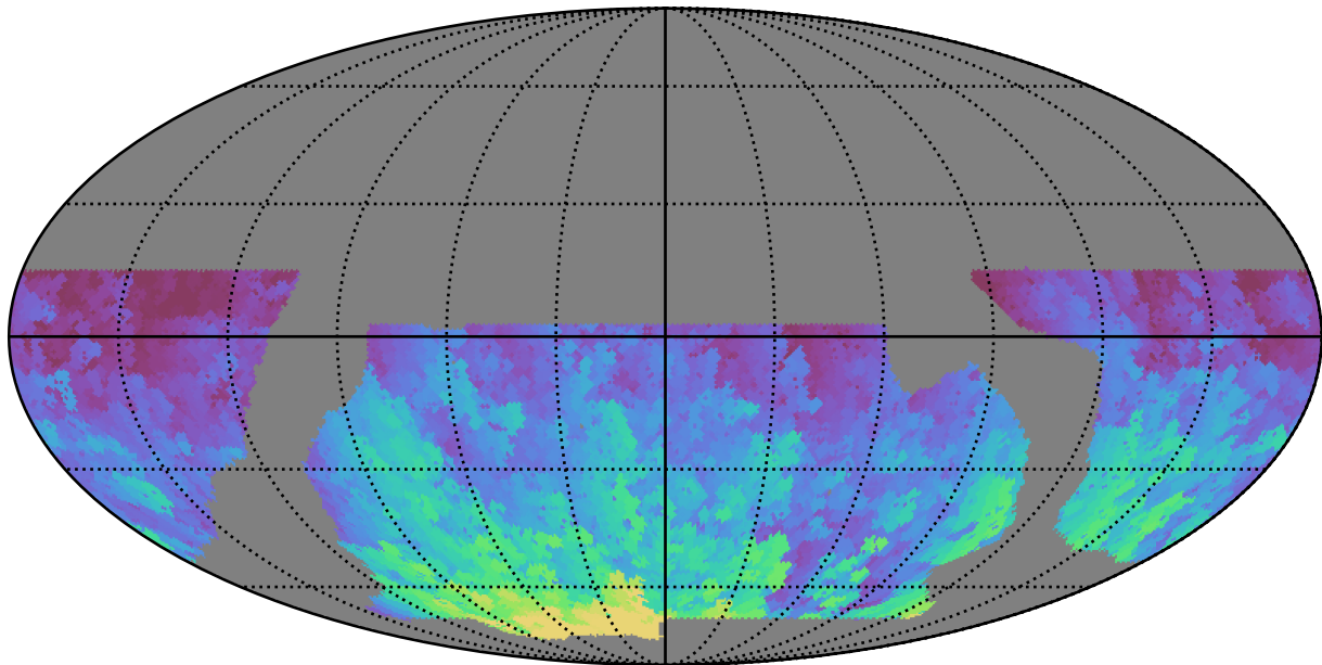
baseline_v2.0_10yrs WFD r band: Max HA
