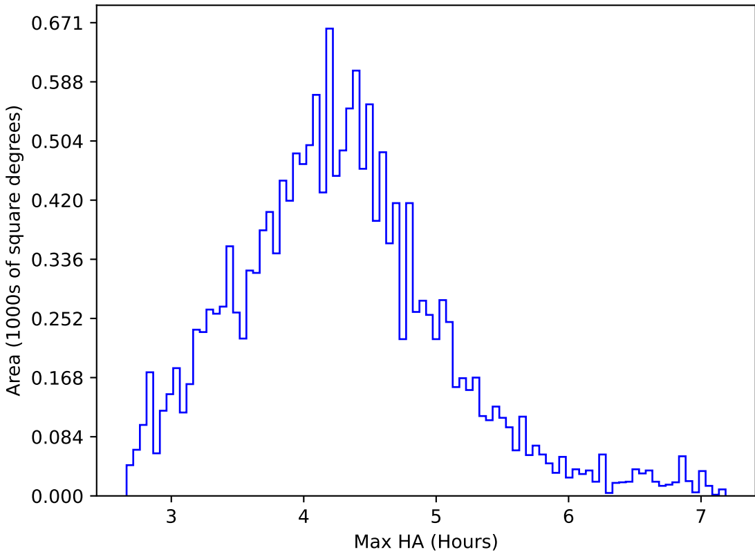
baseline_v2.0_10yrs WFD i band: Max HA
