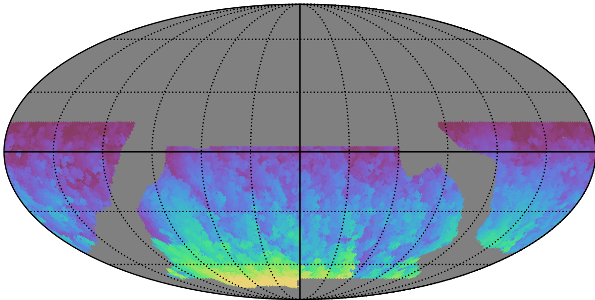
baseline_v2.0_10yrs WFD all bands: Max HA
