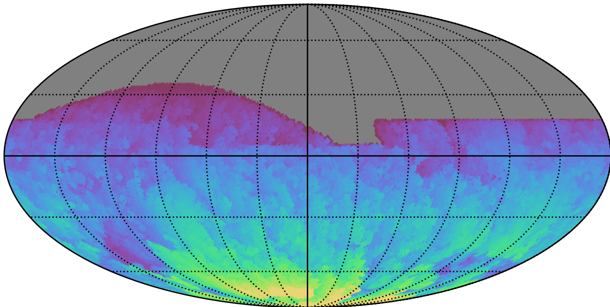
baseline_v2.0_10yrs All sky all bands: Max HA
