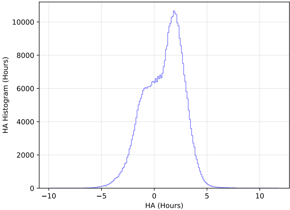
baseline_v2.0_10yrs WFD z band: HA Histogram
