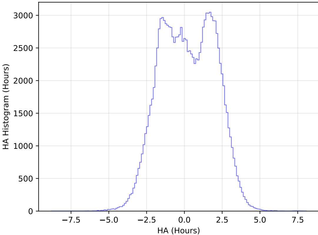
baseline_v2.0_10yrs WFD u band: HA Histogram
