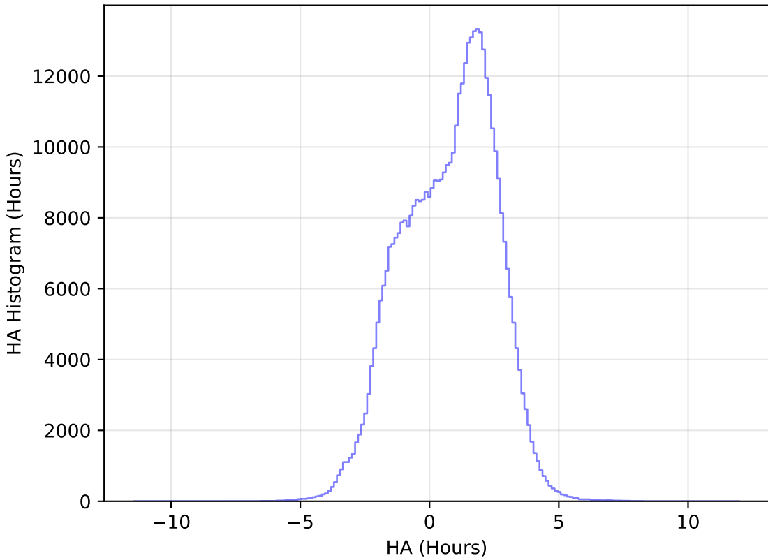
baseline_v2.0_10yrs WFD i band: HA Histogram
