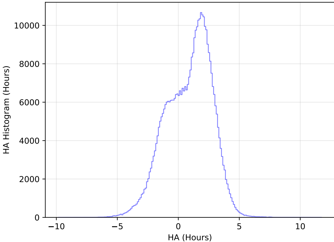
baseline_v2.0_10yrs All sky z band: HA Histogram
