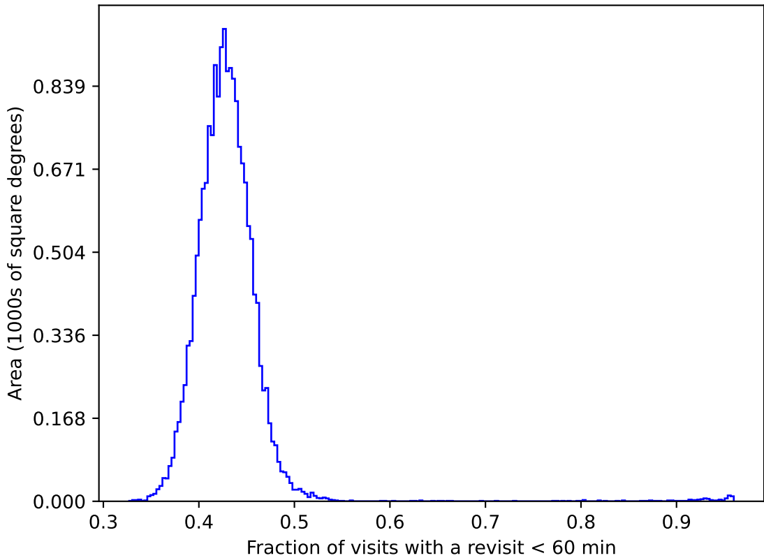
baseline_v2.0_10yrs gri WFD: Fraction of visits with a revisit < 60 min
