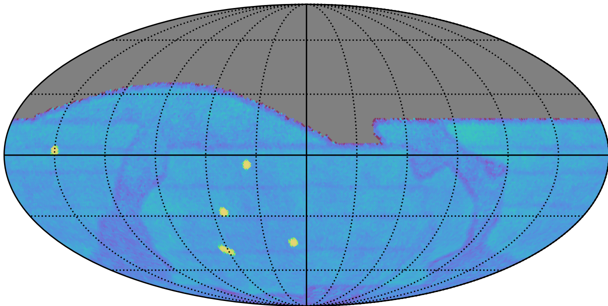
baseline_v2.0_10yrs gri All sky: Fraction of visits with a revisit < 60 min
