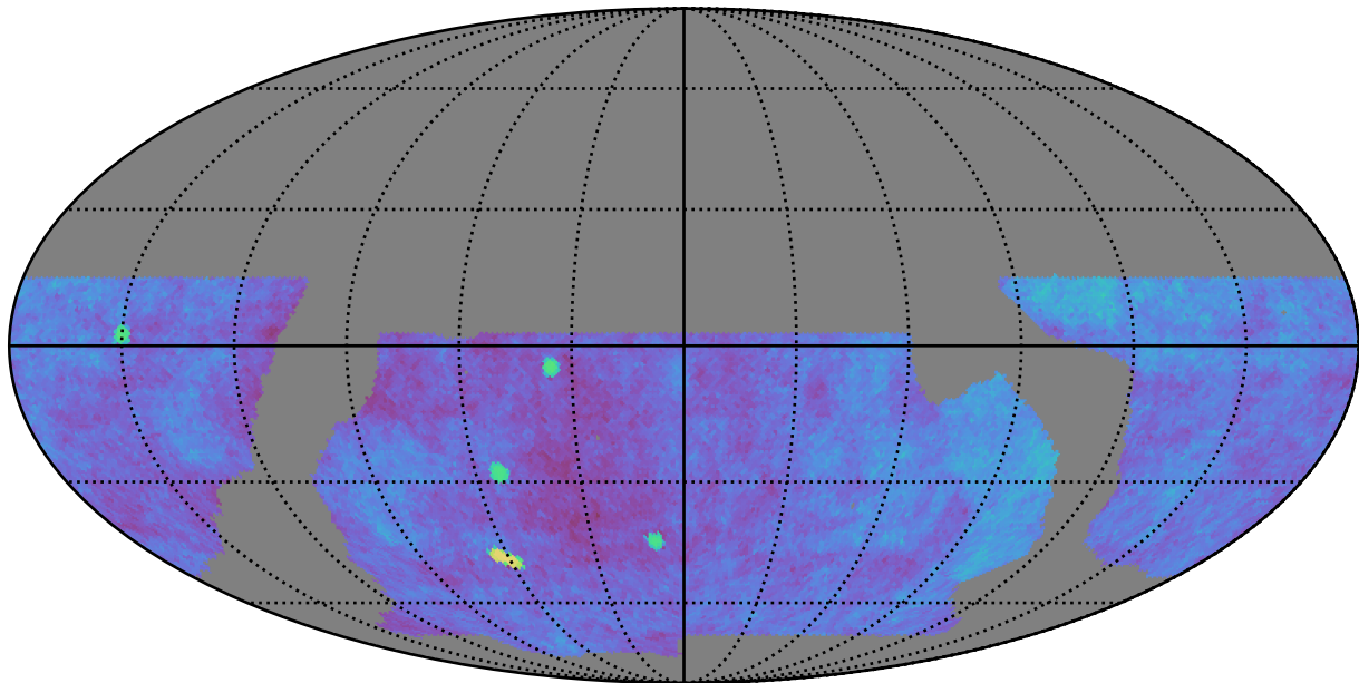
baseline_v2.0_10yrs gri WFD: Fraction of visits in pairs (20-90 min)
