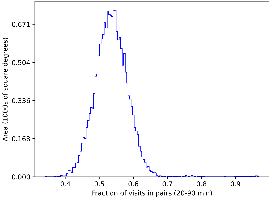
baseline_v2.0_10yrs gri WFD: Fraction of visits in pairs (20-90 min)
