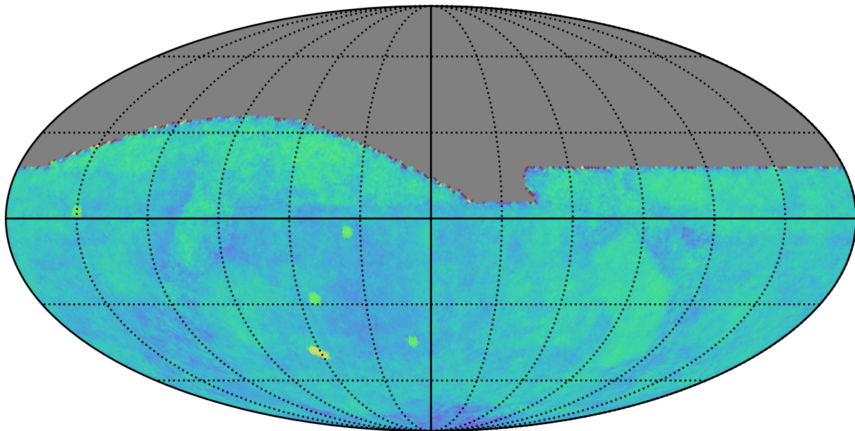
baseline_v2.0_10yrs gri All sky: Fraction of visits in pairs (20-90 min)
