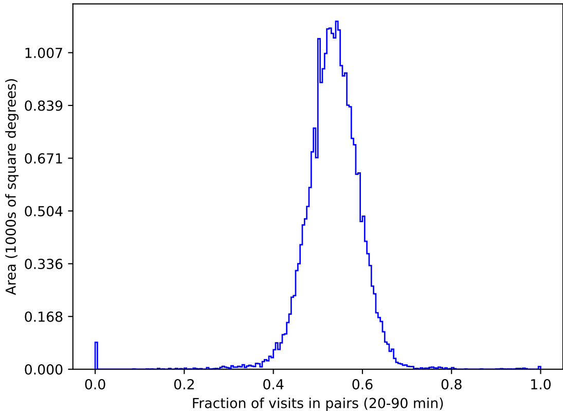
baseline_v2.0_10yrs gri All sky: Fraction of visits in pairs (20-90 min)
