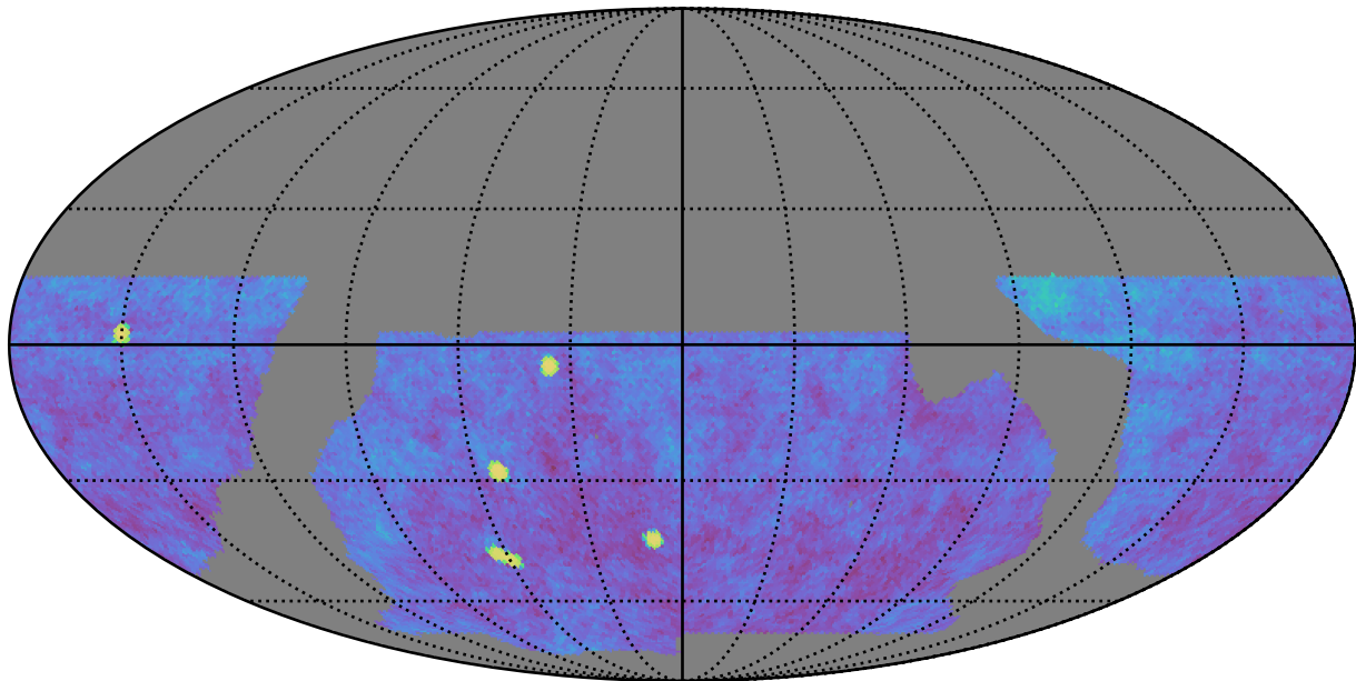
baseline_v2.0_10yrs gri WFD: Fraction of visits in pairs (10-60 min)
