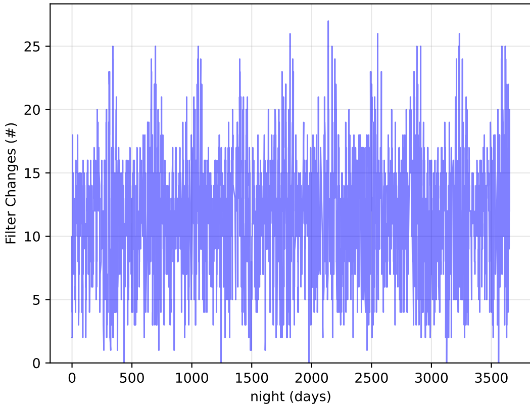
baseline_v2.0_10yrs Per Night: Filter Changes
