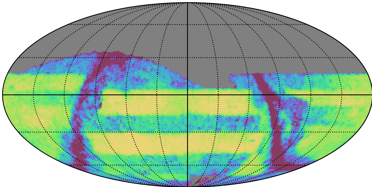
baseline_v2.0_10yrs Yr 3-4 z band: Exgal_CoaddM5
