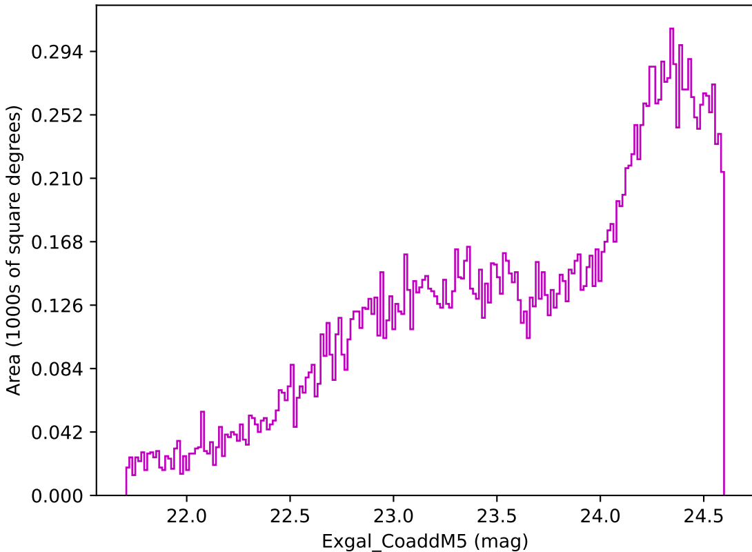
baseline_v2.0_10yrs Yr 3-4 z band: Exgal_CoaddM5
