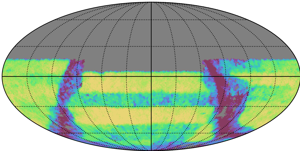
baseline_v2.0_10yrs Yr 3-4 y band: Exgal_CoaddM5
