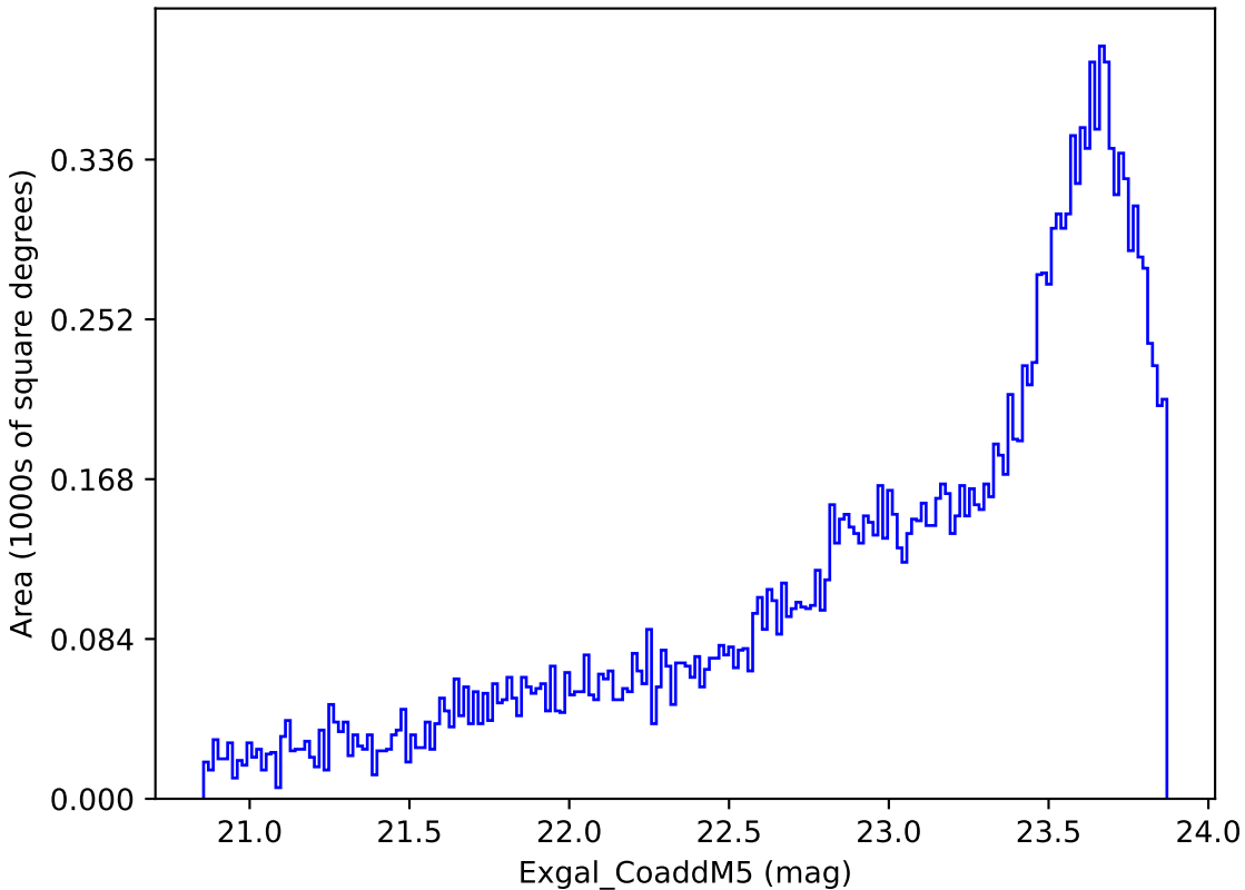
baseline_v2.0_10yrs Yr 3-4 y band: Exgal_CoaddM5
