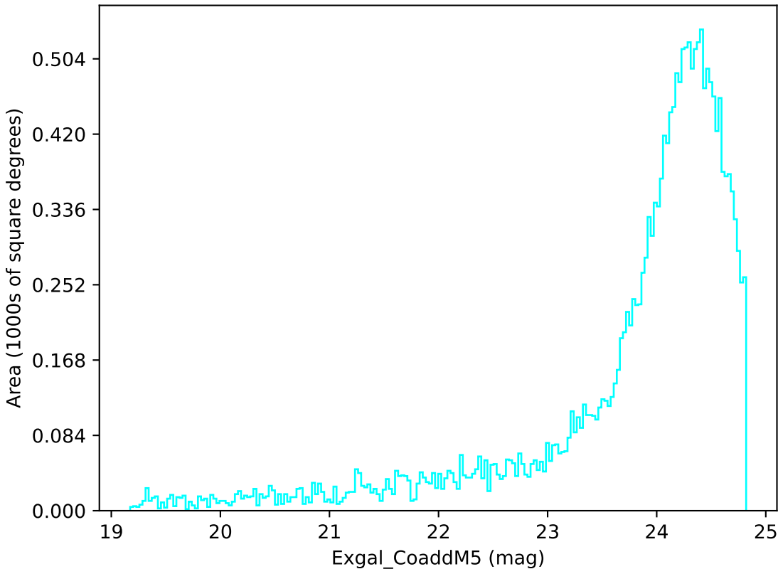
baseline_v2.0_10yrs Yr 3-4 u band: Exgal_CoaddM5
