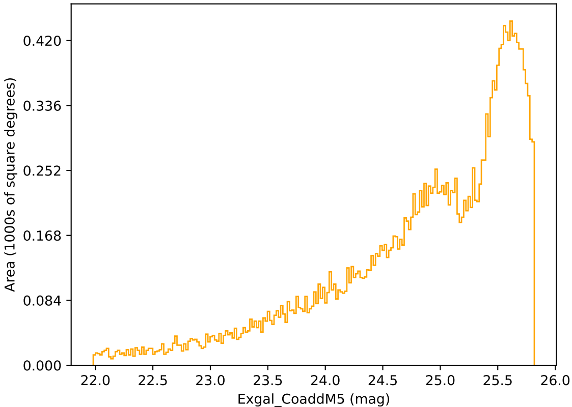
baseline_v2.0_10yrs Yr 3-4 r band: Exgal_CoaddM5
