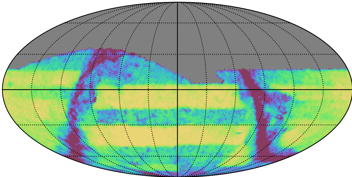
baseline_v2.0_10yrs Yr 3-4 i band: Exgal_CoaddM5
