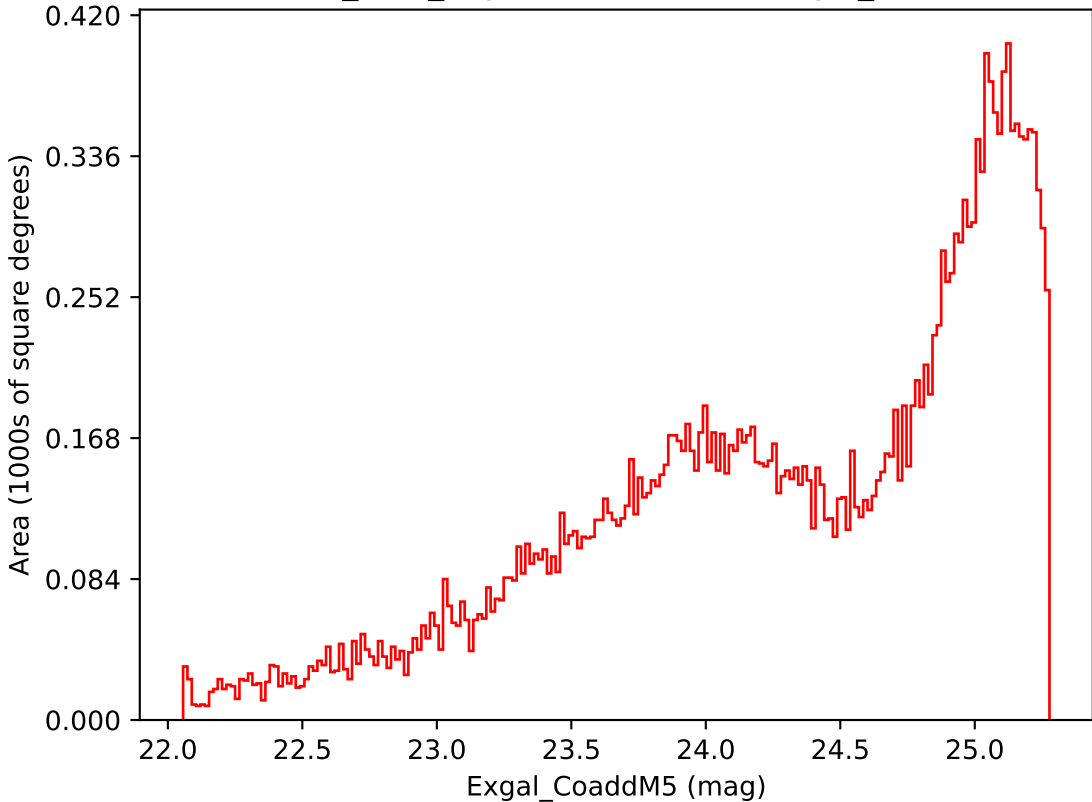
baseline_v2.0_10yrs Yr 3-4 i band: Exgal_CoaddM5
