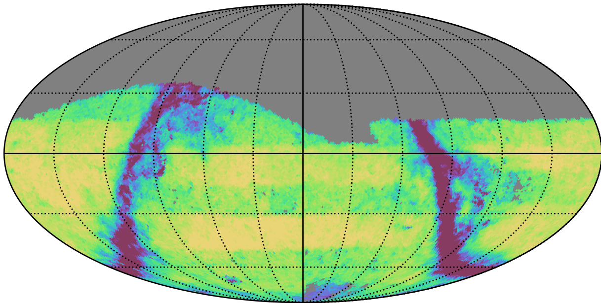
baseline_v2.0_10yrs Yr 3-4 g band: Exgal_CoaddM5
