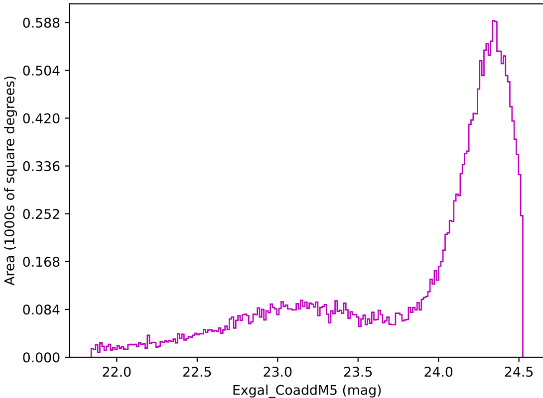
baseline_v2.0_10yrs Yr 1 z band: Exgal_CoaddM5
