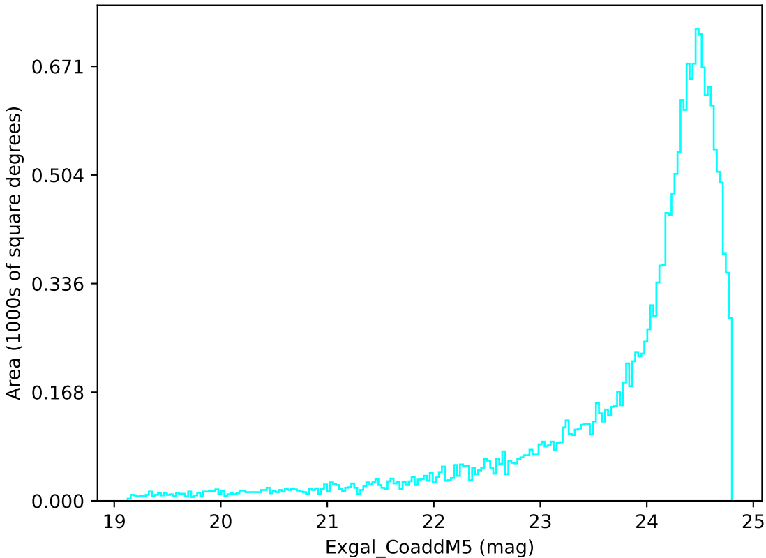
baseline_v2.0_10yrs Yr 1 u band: Exgal_CoaddM5
