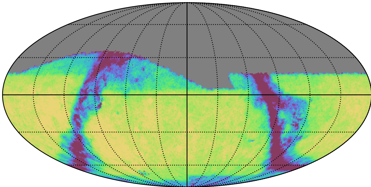
baseline_v2.0_10yrs Yr 1 i band: Exgal_CoaddM5
