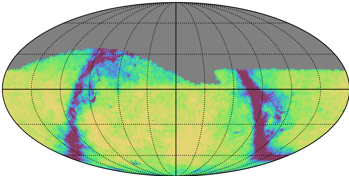
baseline_v2.0_10yrs Yr 1 g band: Exgal_CoaddM5
