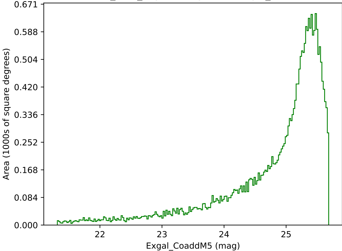
baseline_v2.0_10yrs Yr 1 g band: Exgal_CoaddM5
