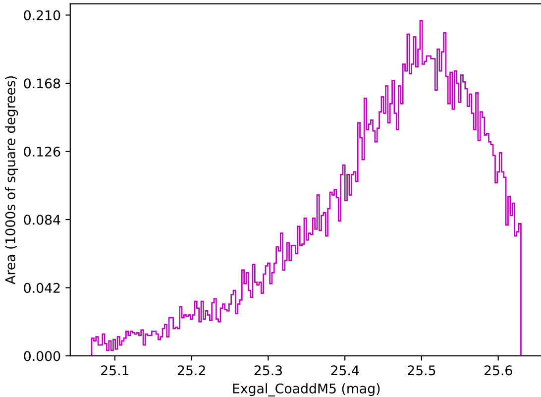
baseline_v2.0_10yrs WFD z band: Exgal_CoaddM5
