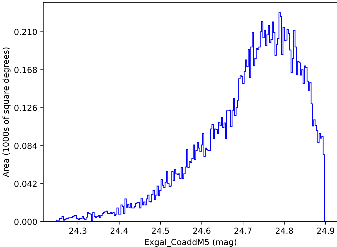
baseline_v2.0_10yrs WFD y band: Exgal_CoaddM5
