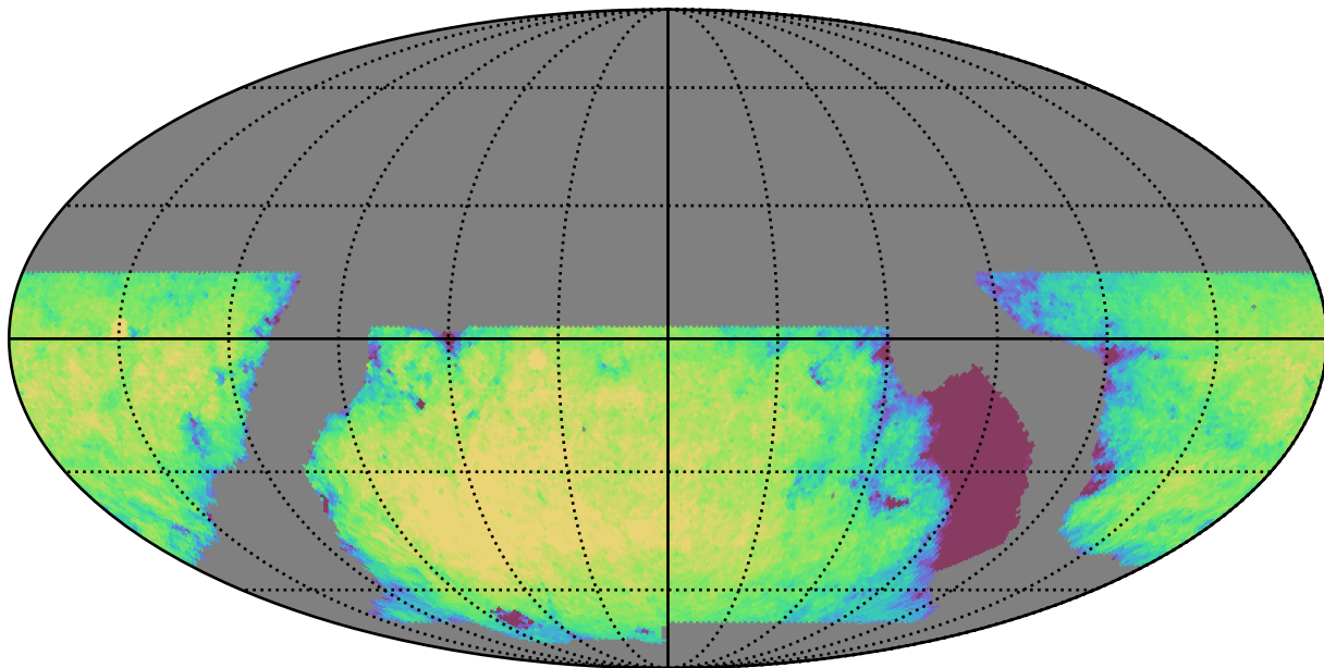
baseline_v2.0_10yrs WFD u band: Exgal_CoaddM5
