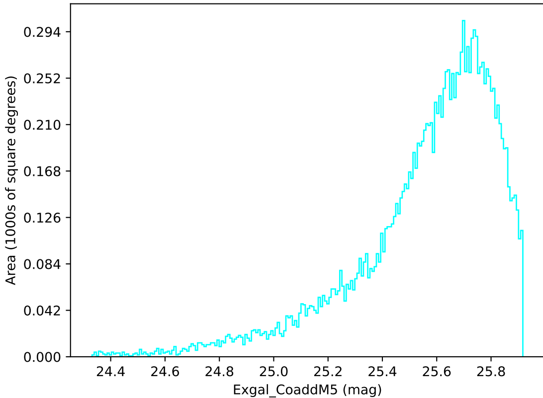
baseline_v2.0_10yrs WFD u band: Exgal_CoaddM5
