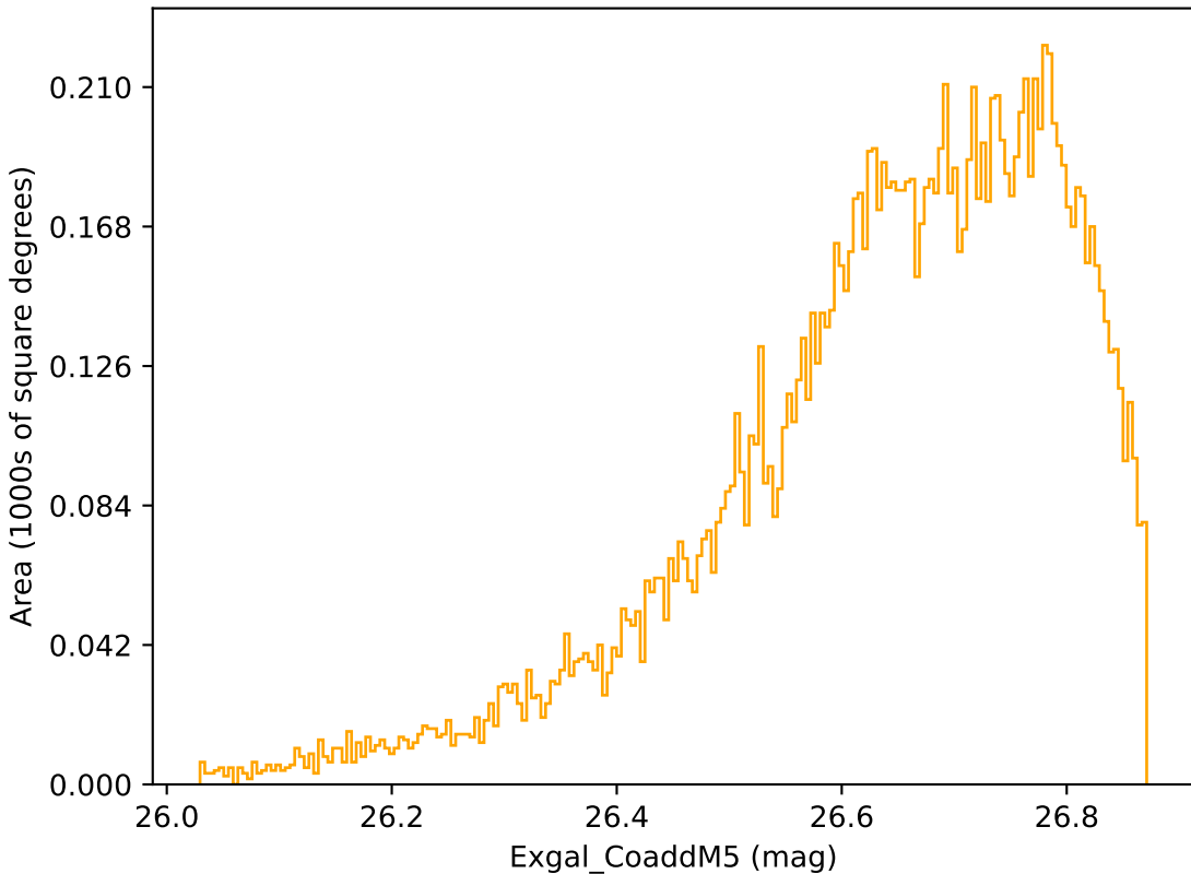
baseline_v2.0_10yrs WFD r band: Exgal_CoaddM5
