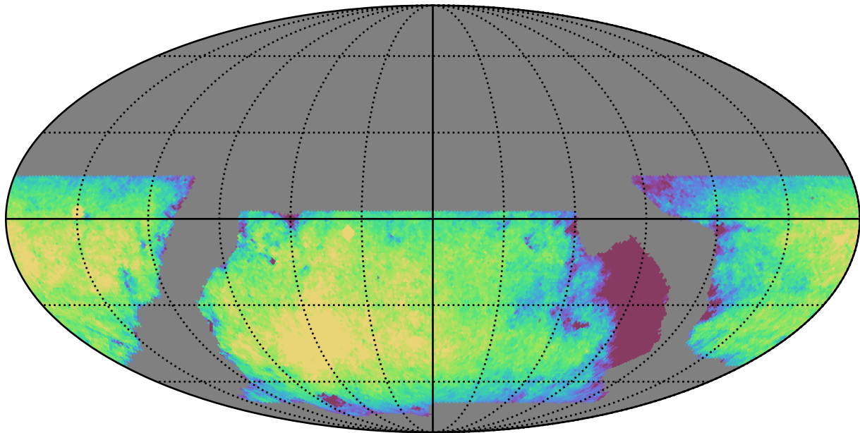
baseline_v2.0_10yrs WFD i band: Exgal_CoaddM5
