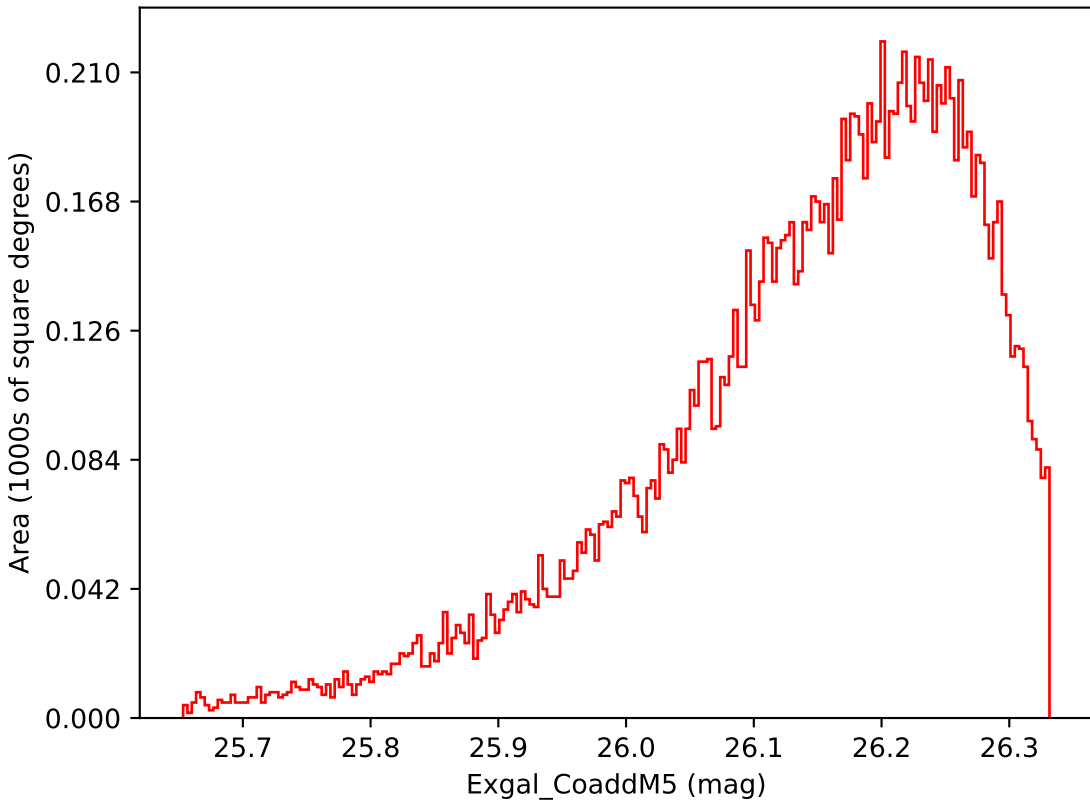
baseline_v2.0_10yrs WFD i band: Exgal_CoaddM5
