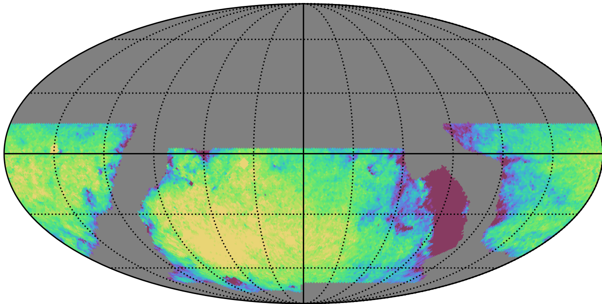
baseline_v2.0_10yrs WFD g band: Exgal_CoaddM5
