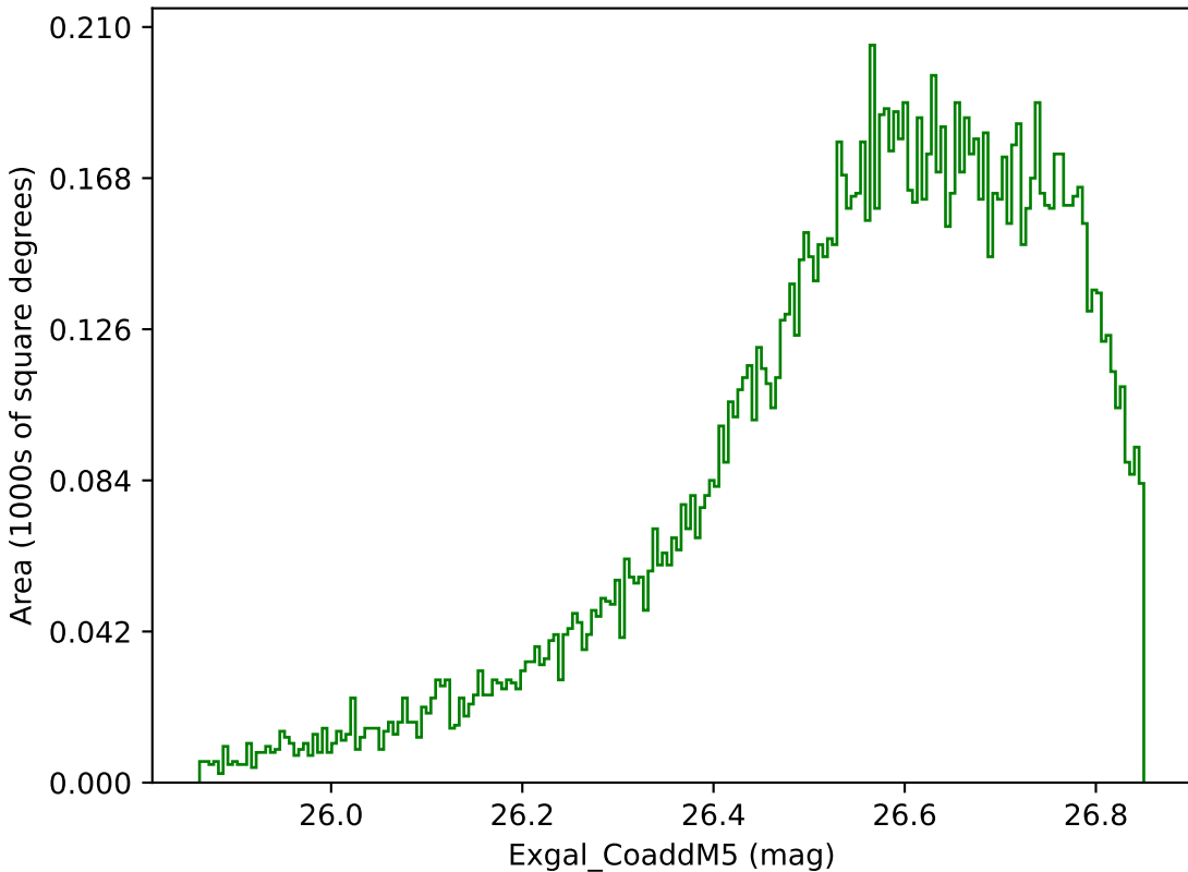
baseline_v2.0_10yrs WFD g band: Exgal_CoaddM5
