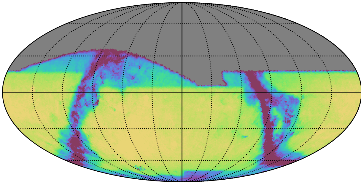
baseline_v2.0_10yrs All sky z band: Exgal_CoaddM5
