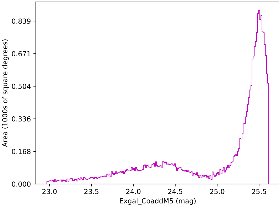
baseline_v2.0_10yrs All sky z band: Exgal_CoaddM5
