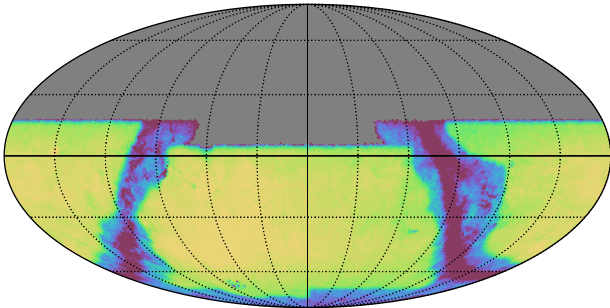
baseline_v2.0_10yrs All sky y band: Exgal_CoaddM5
