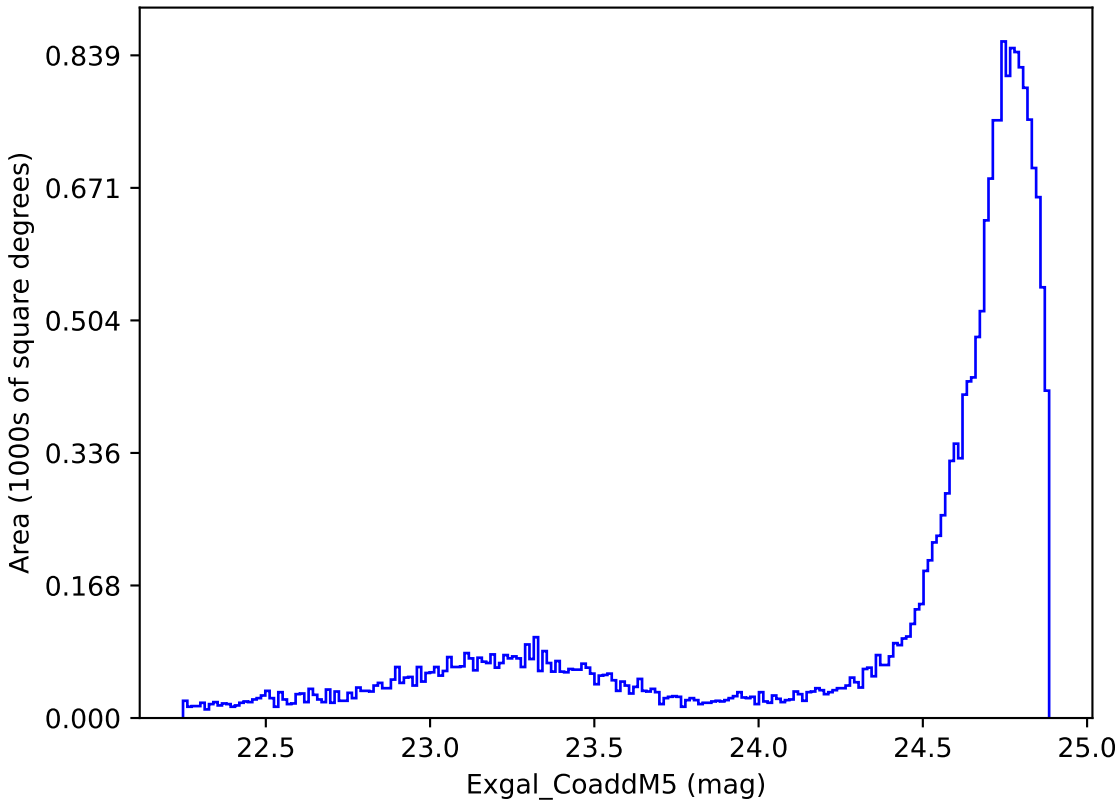
baseline_v2.0_10yrs All sky y band: Exgal_CoaddM5
