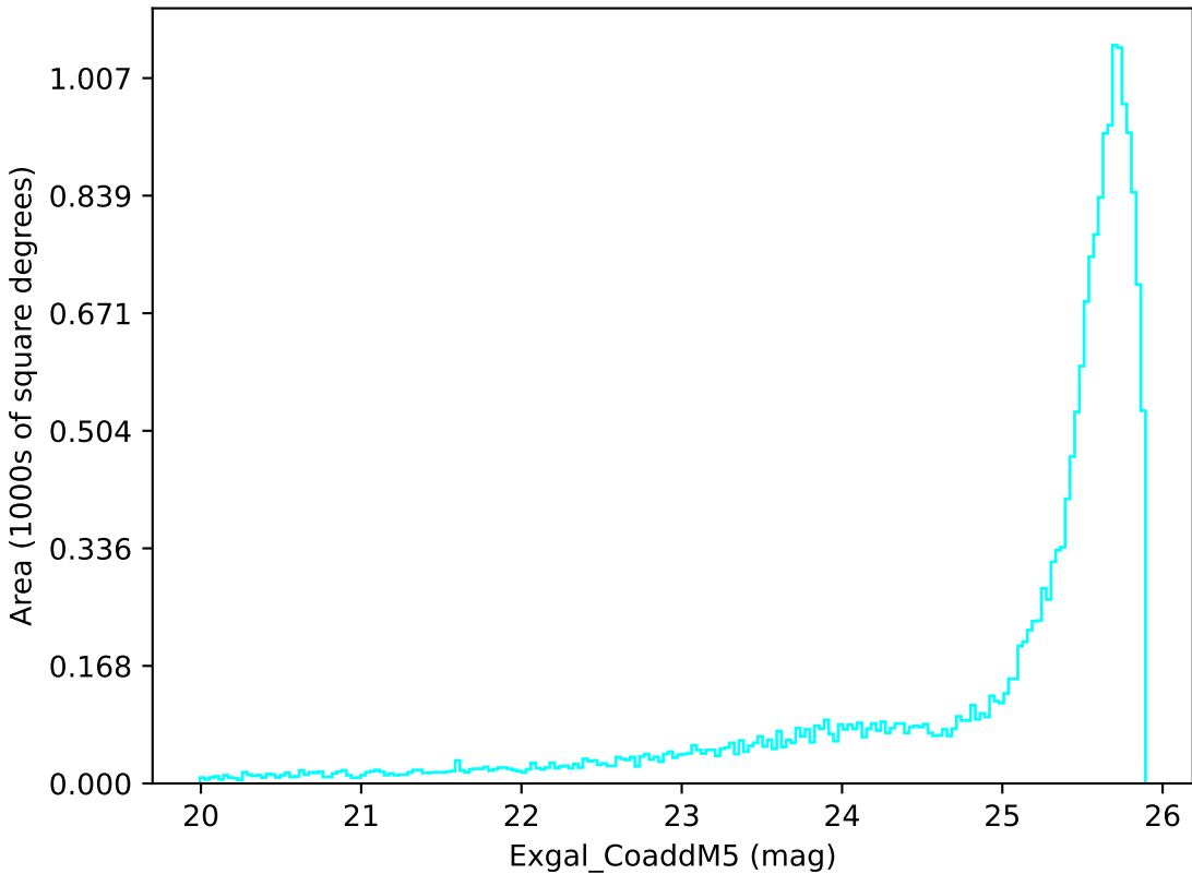
baseline_v2.0_10yrs All sky u band: Exgal_CoaddM5
