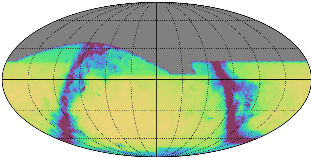
baseline_v2.0_10yrs All sky r band: Exgal_CoaddM5
