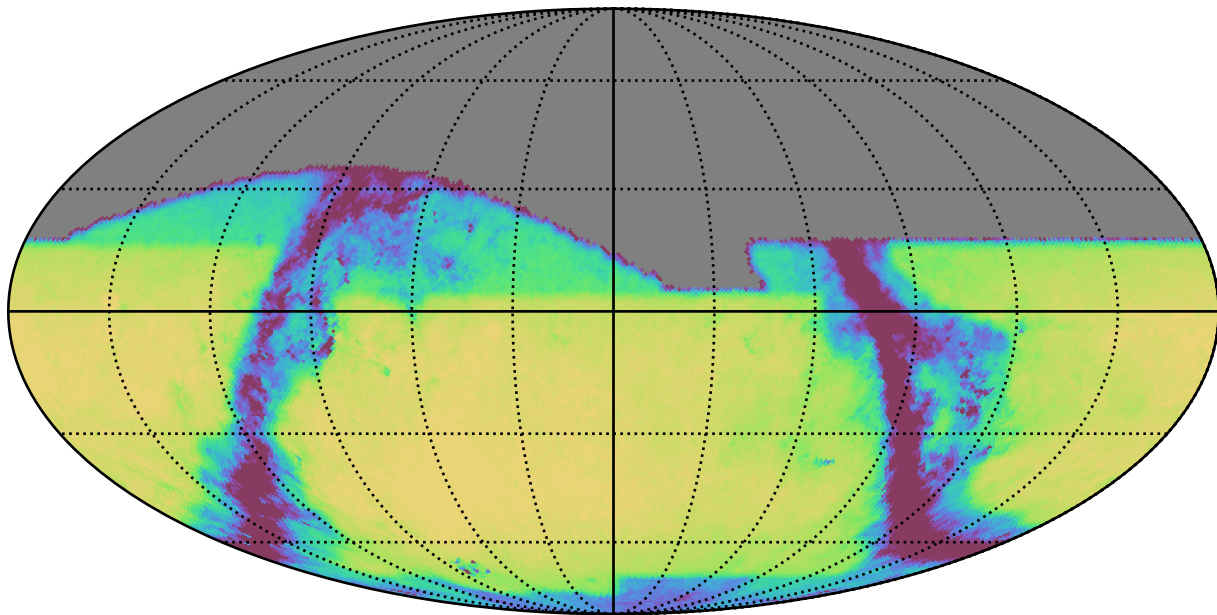
baseline_v2.0_10yrs All sky i band: Exgal_CoaddM5
