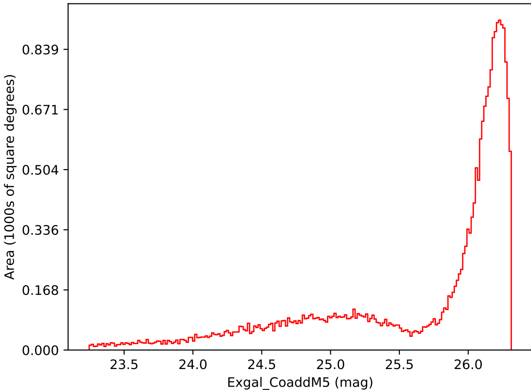
baseline_v2.0_10yrs All sky i band: Exgal_CoaddM5
